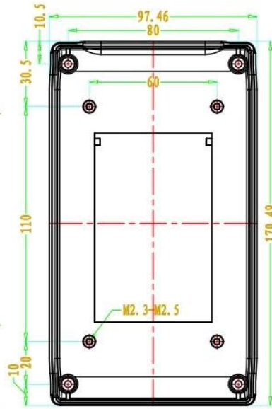
SEC B-B
