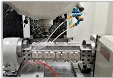
CNC Milling
