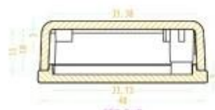
SEC B-B
