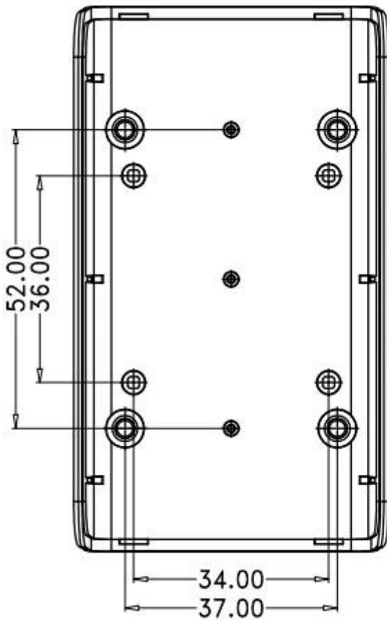
SECTION B-B
