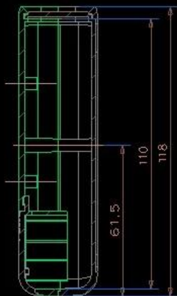
SECTION C—C
