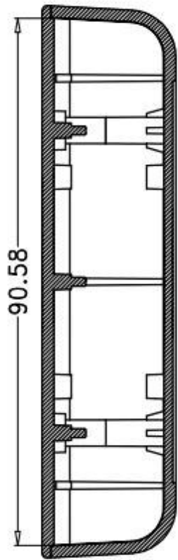
SECTION B-B
