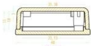
SEC B-B
