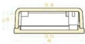
SEC B-B
