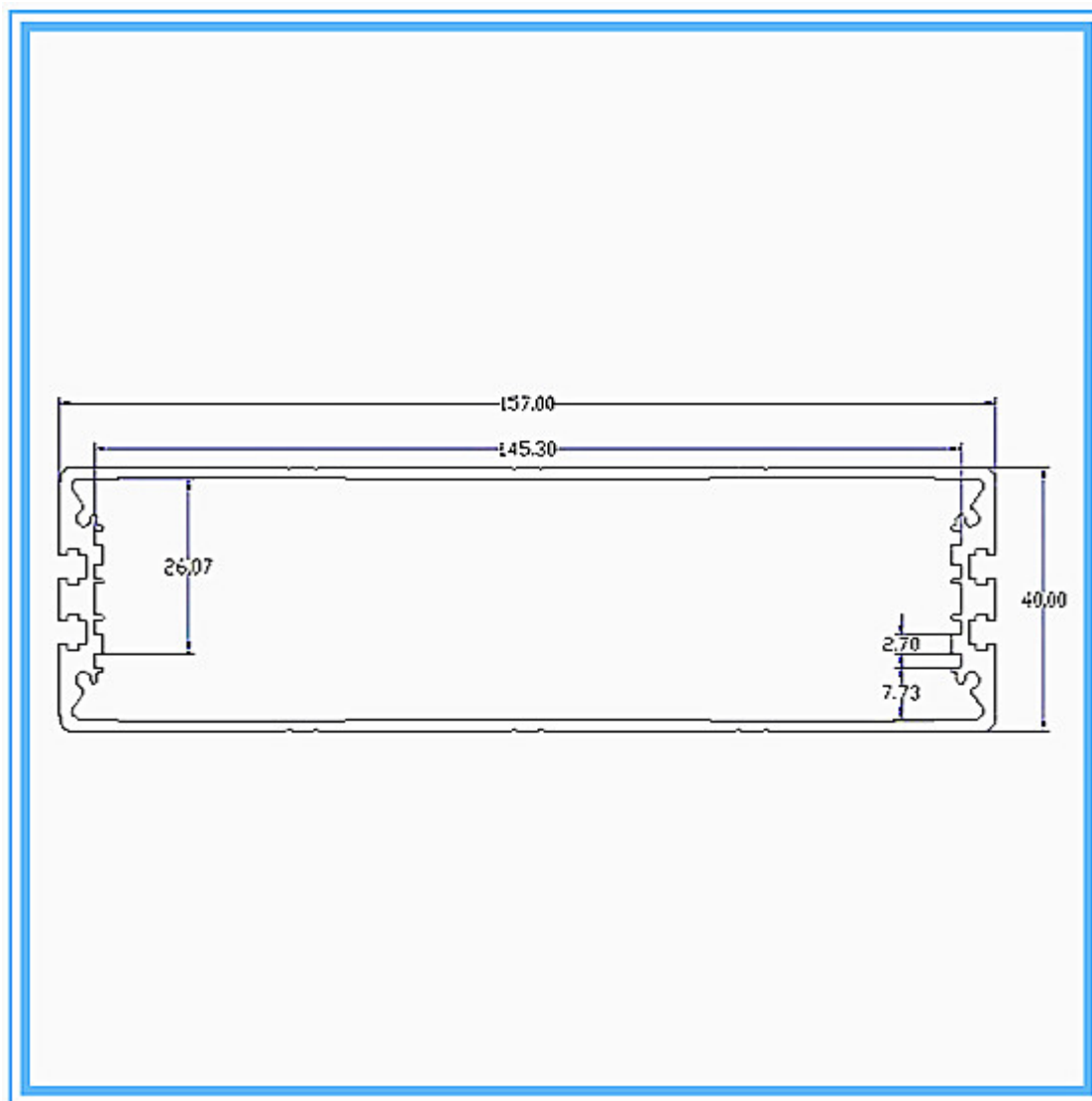
Wandmontage serie aluminium behuizing
