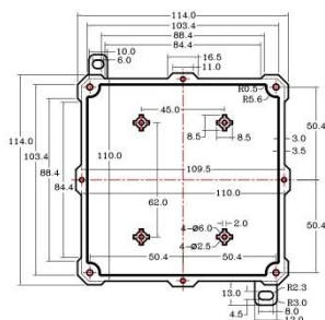
AK-BW-07 114*114*62mm
