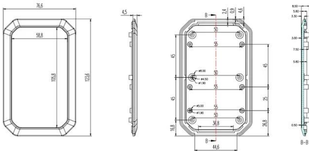
AK-H-77 Drawing
