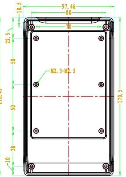
SEC B-B
