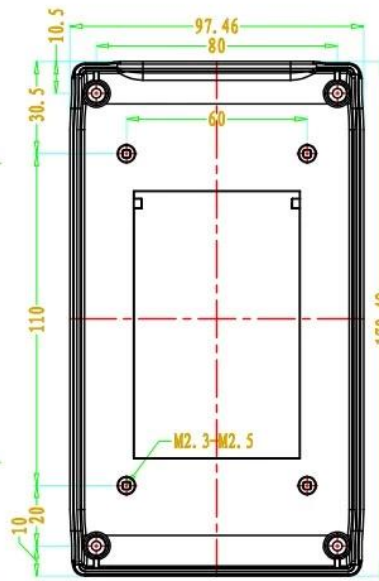
SEC B-B
