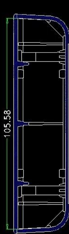
SECTION B-B
