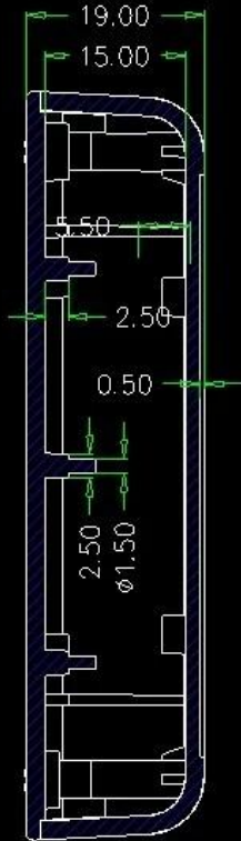
SEC B-B
