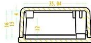
SEC B-B
