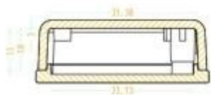
SEC B-B
