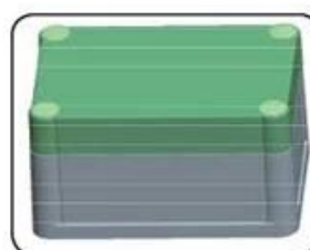
Gasket (1PCS) Material:Rubber Size:96.5*64.5*1.8 mm
