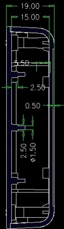
SEC B-B
